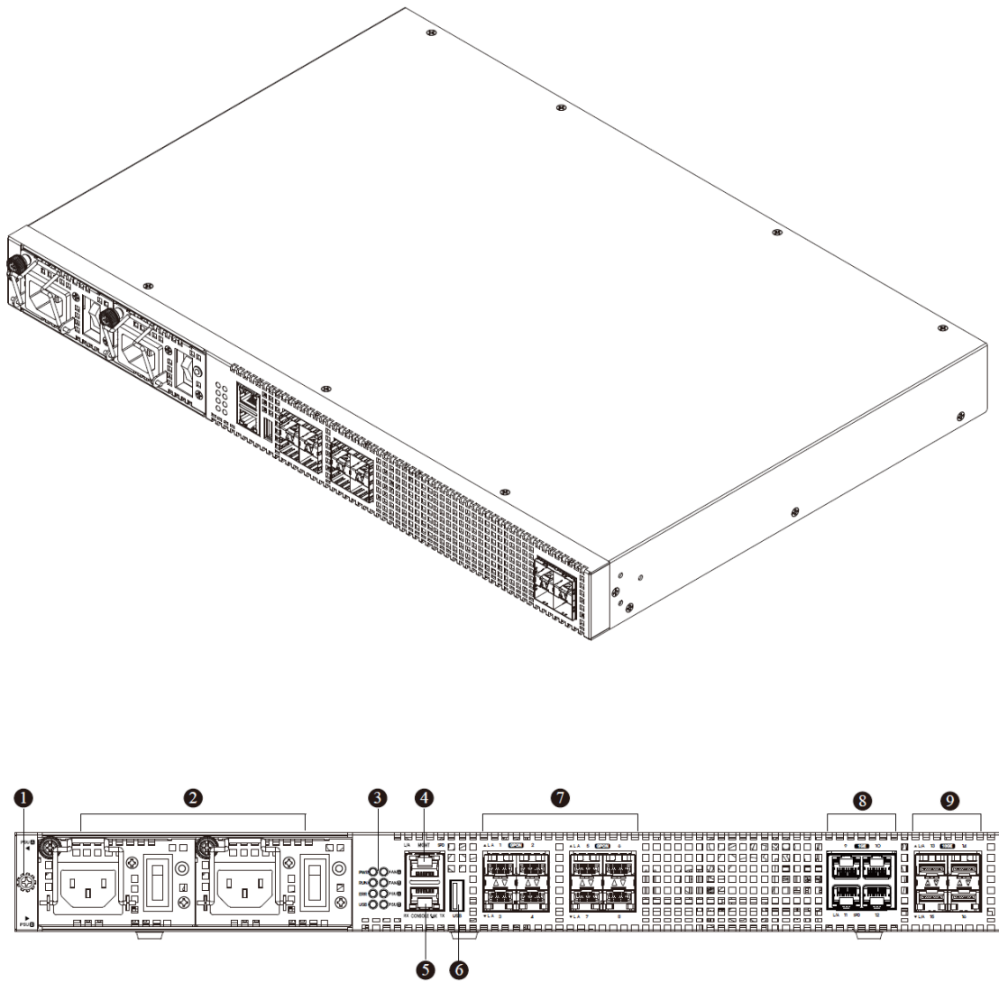
Figure 1 Front View of V5808
