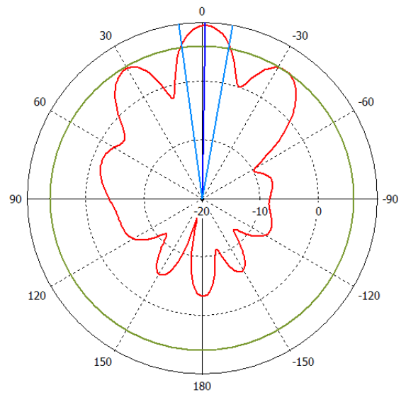
HP elevation
