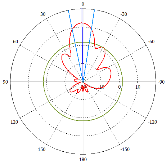
VP elevation
